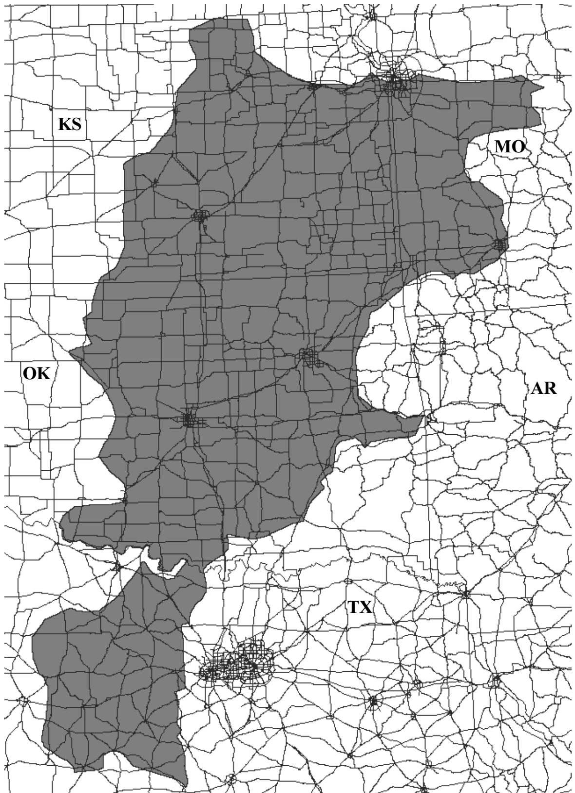
Road network in the Osage Plains, physiographic area 33.
