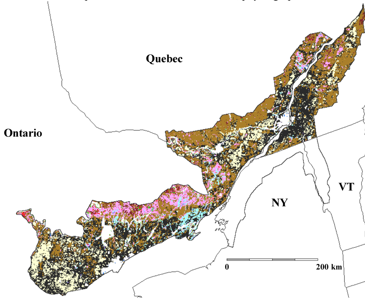
Forest types in the Canadian portion of the St. Lawrence Plain, physiographic area 18, from CCRS data
