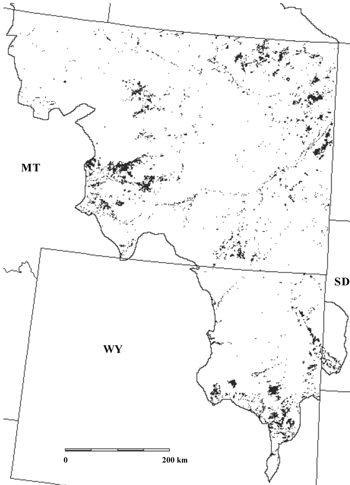
Grama grassland in the U.S. portion of the Northern Shortgrass Prairie, physiographic area 39, covering 1,379,200 ha (3,408,003 ac), or 3.23% of the area.
