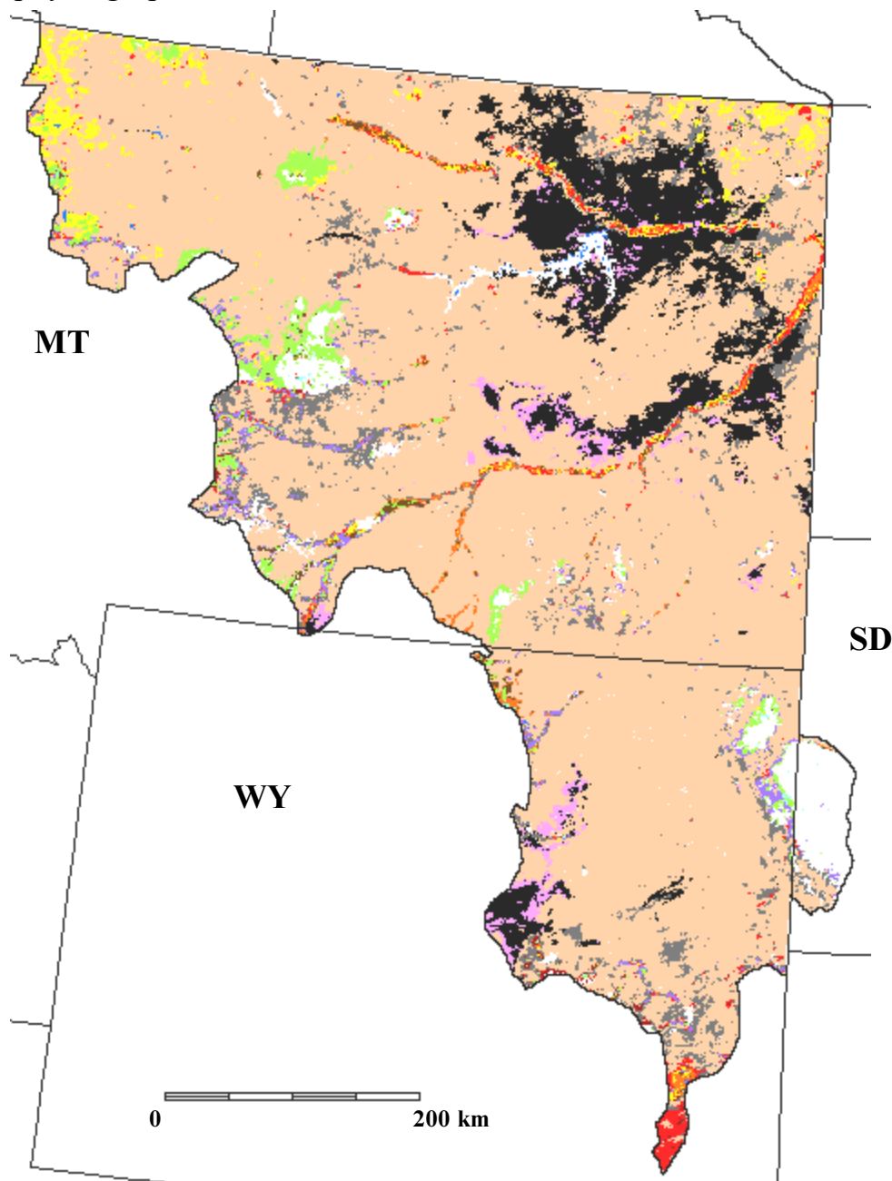
Forest and nonforest cover types in the U.S. portion of the Northern Shortgrass Prairie, physiographic area 39, modified from USGS data.
