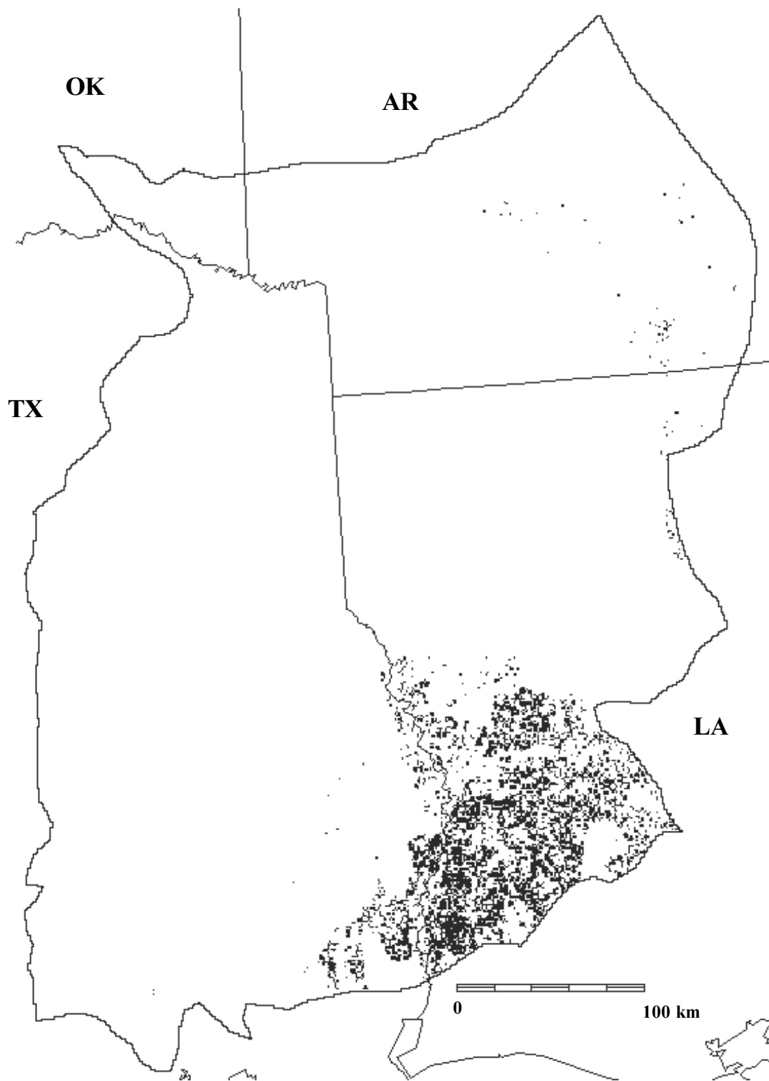
Longleaf-slash pine forests in the West Gulf Coastal Plain, physiographic area 42, covering 529,079 ha (1,307,355 ac), or 3.52% of the area.
