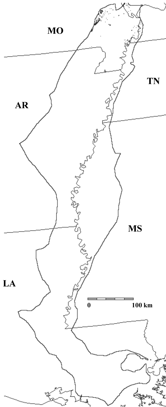
Elm-ash-cottonwood, maple-beech-birch forest in the Mississippi Alluvial Valley, physiographic area 5, covering 31,300 ha (77,342 ac), or 0.27% of the area.
