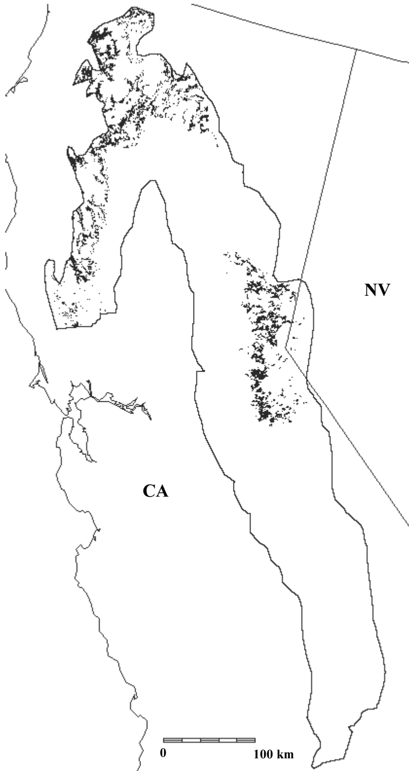
Douglas fir forests in the Sierra Nevada, physiographic area 66, covering 604,400 ha (1,493,472 ac), or 6.21% of the area.
