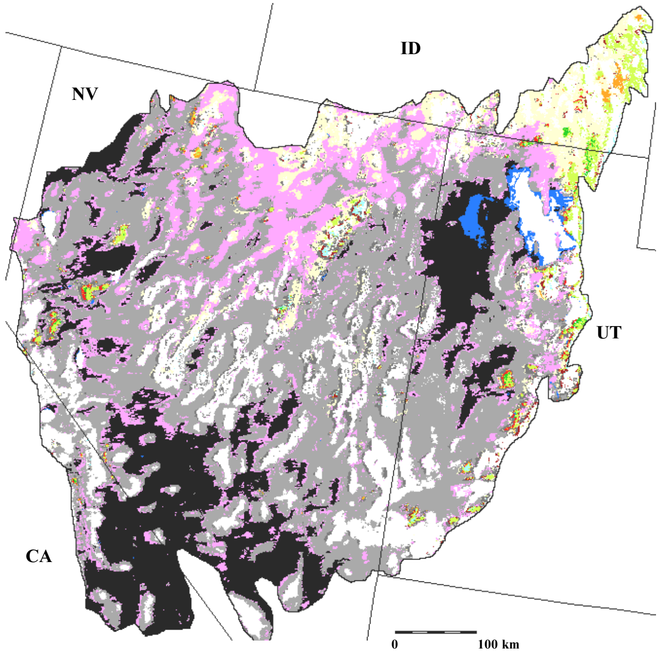
Forest and nonforest cover types in the Basin and Range, physiographic area 80, modified from USGS data.
