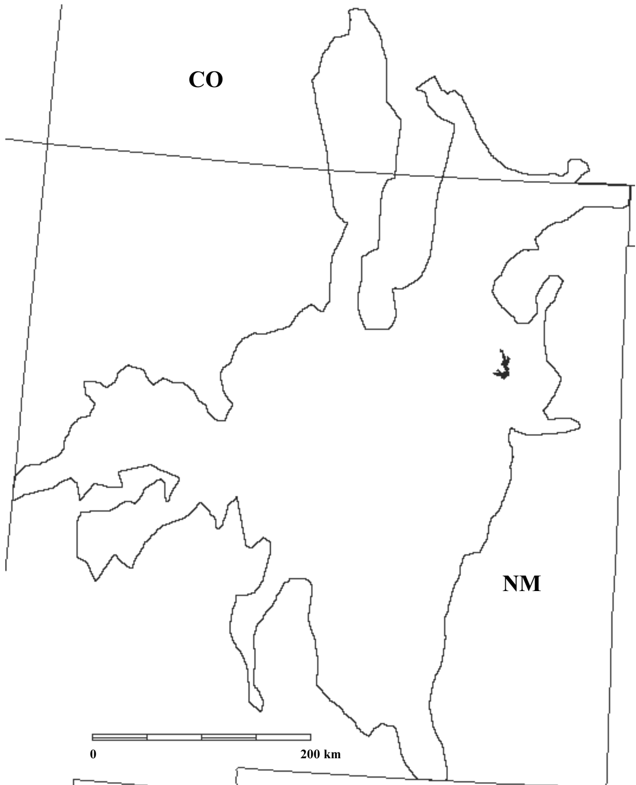
Water in the New Mexico Mesa and Plains, physiographic area 85, covering 15,100 ha (37,312 ac), or 0.12% of the area.
